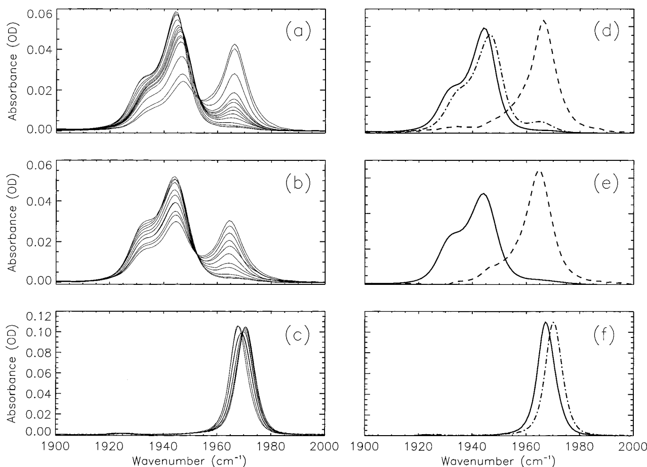
FIGURE 1 Left column: CO stretch infrared spectra in the pH range from 4.2 to 9.5 of (a) swMbCO, (b) proximal mutant H97F, and (c) distal mutant H64L, baseline corrected and normalized to an integrated area of 1 OD \text{cm}^{-1} . Right column: Basis spectra of the different protonation states as determined by least squares fits of the spectra to a model described in the text; (d) swMbCO, with neutral form S_{00} (—), mixed protonation state S_{[01]} (---), and doubly protonated protein S_{11} (- · - ·); (e) H97F, with neutral H64, S_{0x}^{H97F} (—) and protonated H64, S_{1x}^{H97F} (---); (f) H64L, with neutral H97, S_{x0}^{H64L} (—), and protonated H97 S_{x1}^{H64L} (---).
